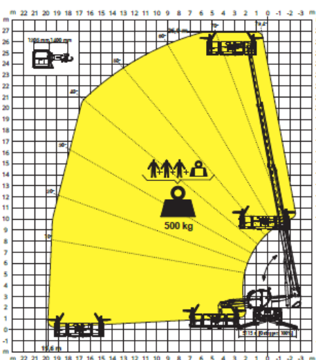
NACELLE EXTENSIBLE ROTATIVE 500 kg
